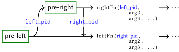
Figure 8. Spawning two processes (green boxes represent spawned concurrent processes)
